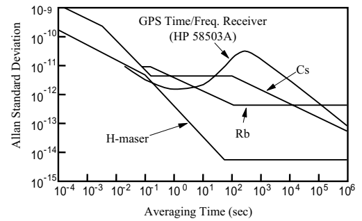
Figure 1. Stability characteristics of GPS time-and-frequency reference receiver, hydrogen maser clock, cesium clock, and rubidium clock.
