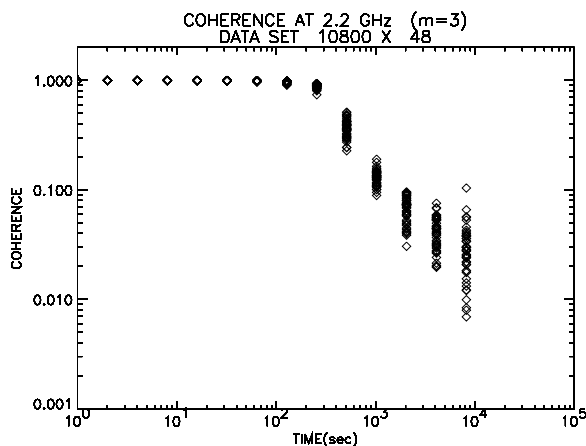
Figure 9. Coherence calculated using residual phase data after third-order polynomial fitting versus integration time for 2.2 GHz
