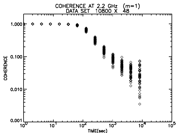
Figure 7. Coherence calculated using residual phase data after removing linear drift versus integration time for 2.2 GHz
