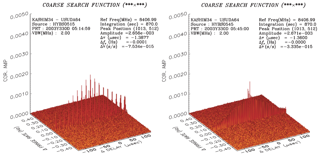
Figure 4. Detected HAYABUSA group delay fringes for the Kashima 34m – Usuda 64m baseline on November 26, 2003. (left: range signal, right: telemetry signal)
