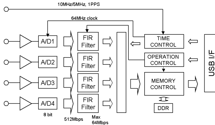
Figure 1. A block diagram of K5/VSSP32 sampler.
