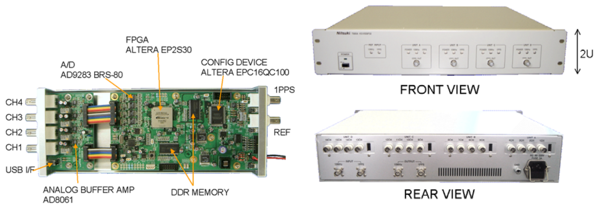
Figure 2. A picture of K5/VSSP32 unit (left) and 16-ch K5/VSSP32 module (right).
