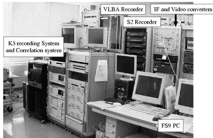
Figure 1. A K5 system located in observation room of 34m station. Since the K5 system is composed from a cluster of PCs, those PCs are used for both observation and correlation processing.
