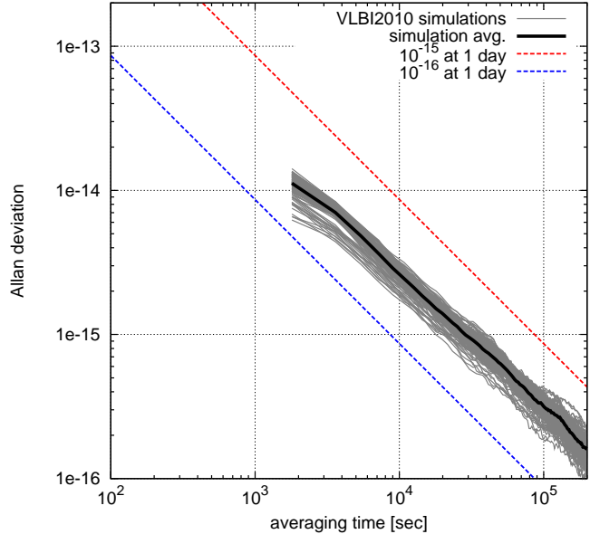
Figure 1. Frequency transfer performance over an 18 station global network of VLBI2010-like stations using a combination of 3m and 10m dishes. Simulated observations were kindly provided from Vienna University of Technology.
