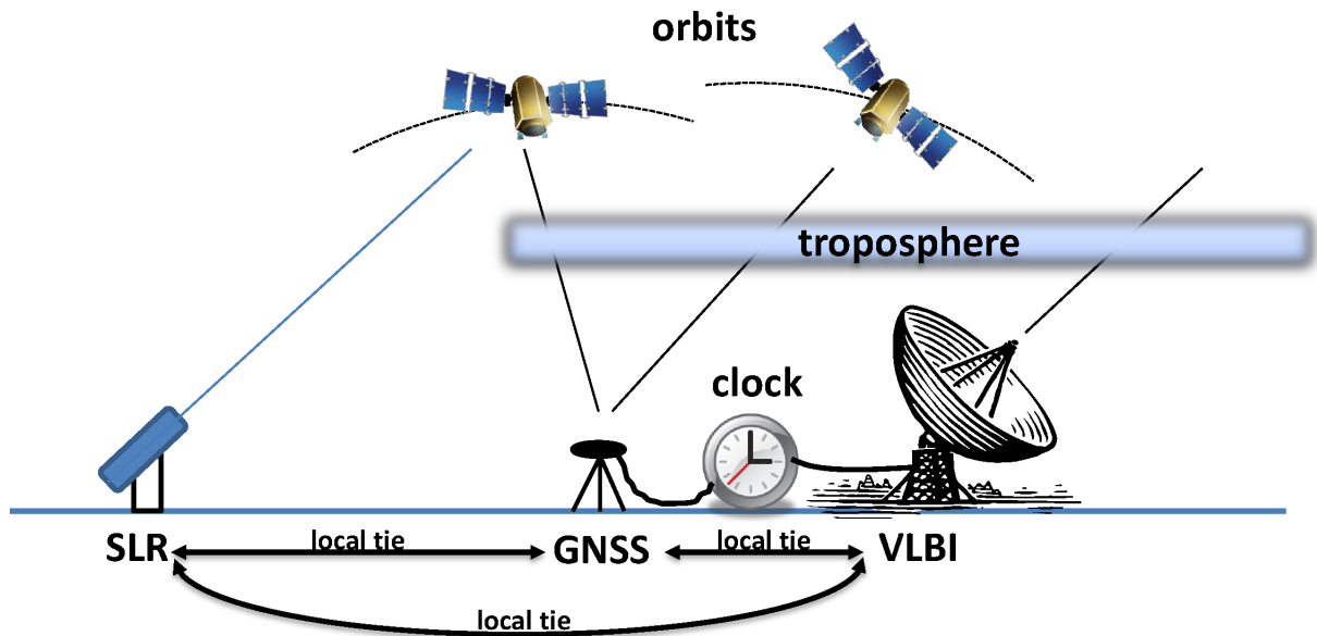
Figure 1. Combination of space-geodetic data on the observation level requires the knowledge of precise local tie information. Co-located VLBI and GNSS technology often shares the same frequency standard, which allows to estimate a single clock model for both techniques. In addition troposphere delays are thought to be identical except a constant bias (so-called "troposphere tie").
