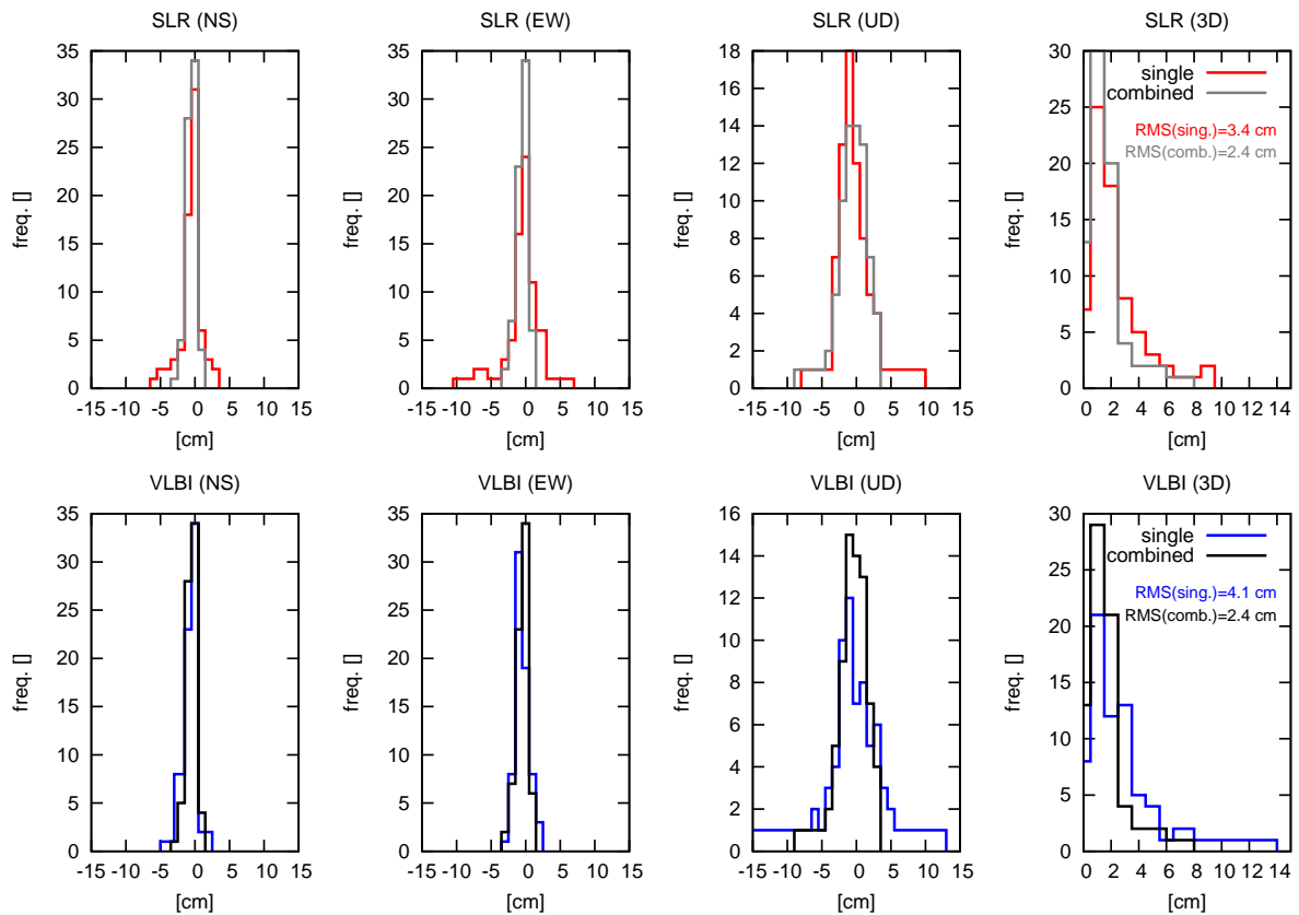
Fig. 2 Histograms of the detrended coordinate time series of the single technique and combined solutions between Jan 1st, 2008 and March 10th (i.e. the occurrence of the Chile 2010 earthquake) as discussed in [3].
