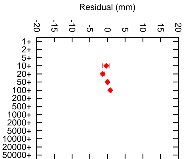
Greenbelt 7105 AJI
