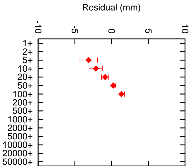
Greenbelt 7105 STRL+STEL
