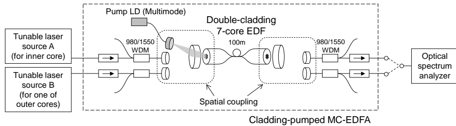
Cladding-pumped MC-EDFA
