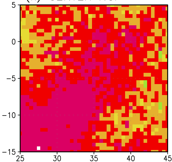
(k) CENTER NCP
