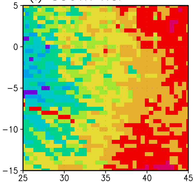
(l) SOUTH NCP
