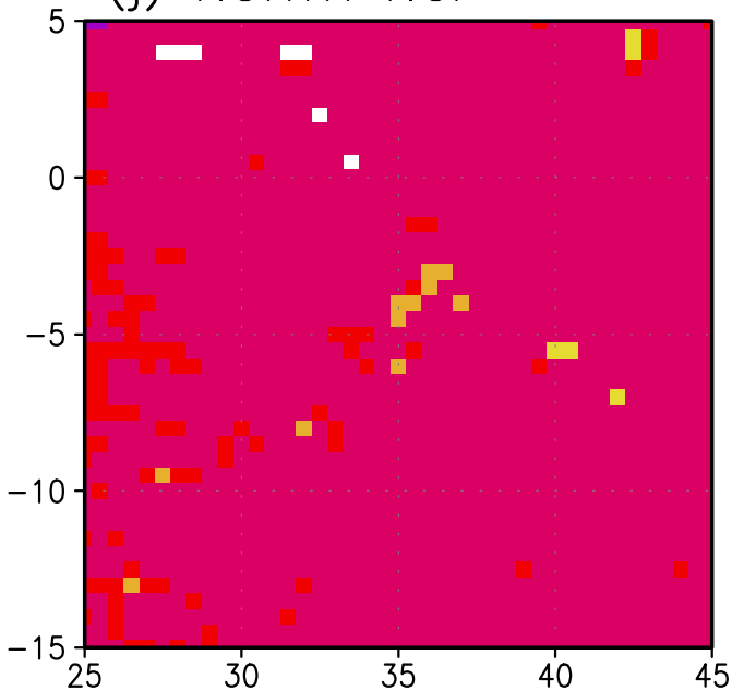
(j) NORTH NCP
