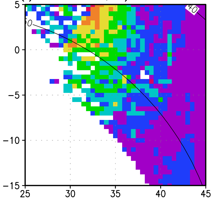
(i) Dif.MAG*du,dv): SO-COMP
