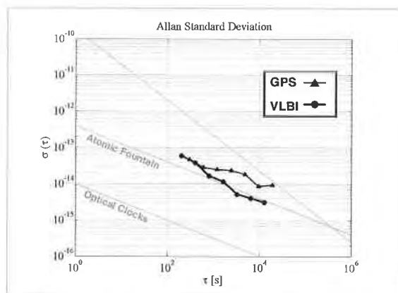
Fig.2 Frequency stability calculated from VLBI and GPS results
