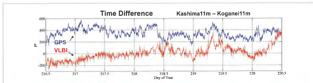
Fig.5 Time difference in August 2010 experiments Kashima 11m–Koganei 11m baseline
