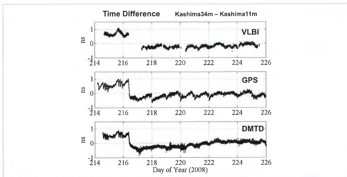
Fig.4 The time difference results of the 3 techniques: VLBI, GPS and DMTD Kashima 34m–Kashima 11m baseline
