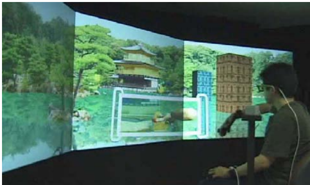
図1 Scope-Based Interaction
